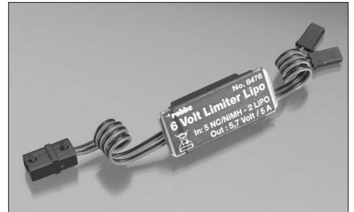
6-VOLT-LIMITER LITHIUM
